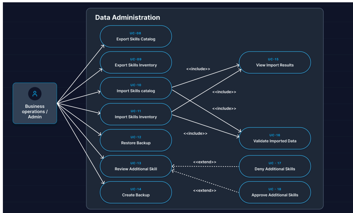
Figure 1: Use Case Model for Data Administration
