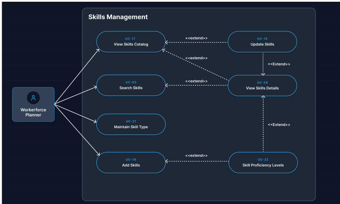
Figure 3: Use Case Model for Workforce Planner
